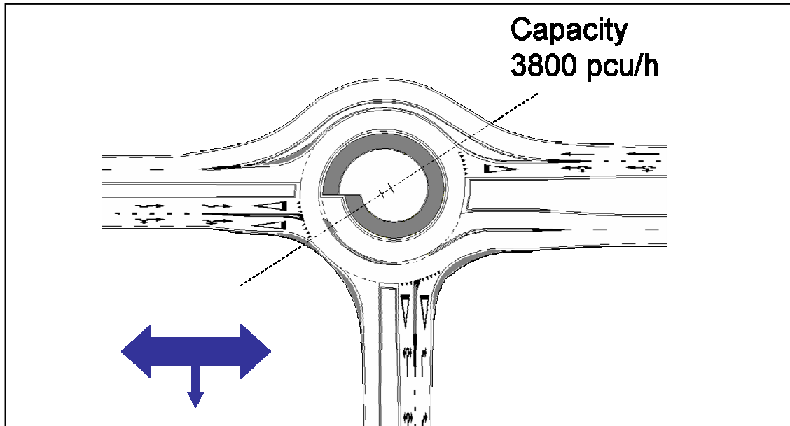
Figure 54: Stretched-knee roundabout
