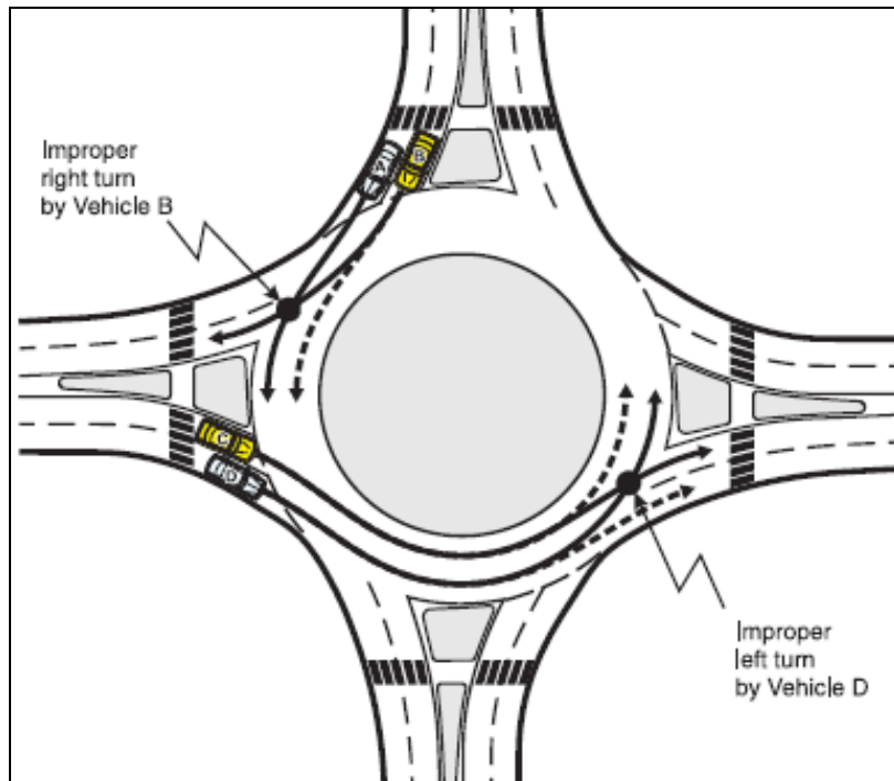
Figure 43: Improper turn conflict at multi lane roundabout [12]
