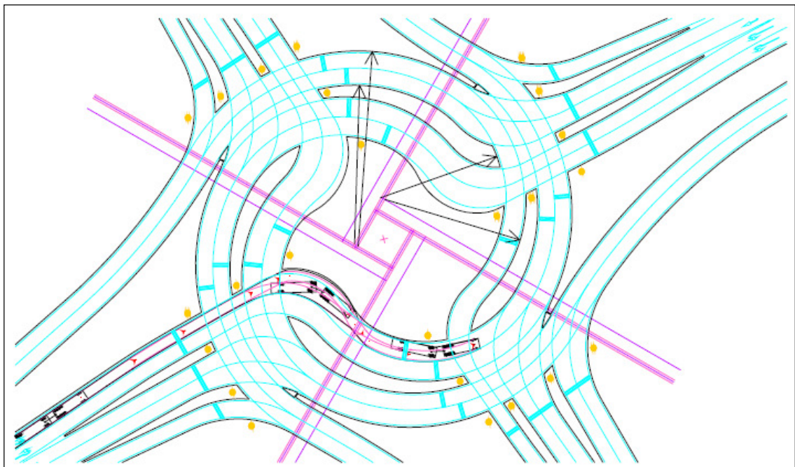
Figure 82: Concept design of a signalized turbo roundabout
