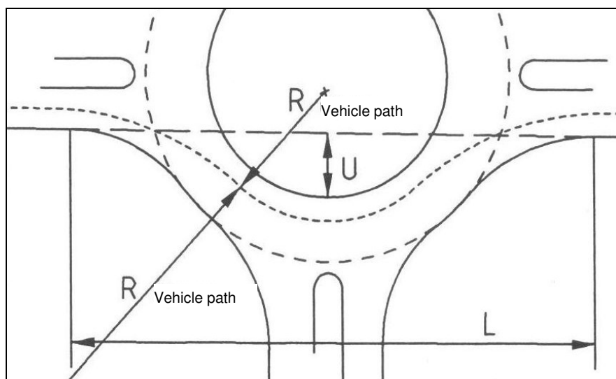
Figure 23: Speed depends of deflection
