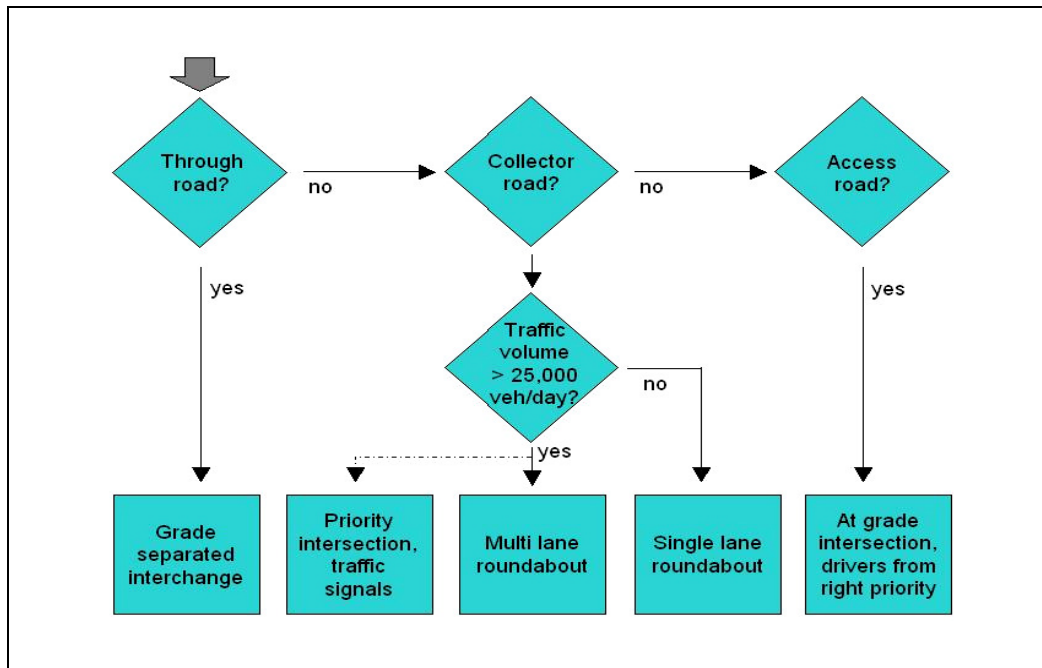
Figure 4: Simplified flow chart choice of intersection
