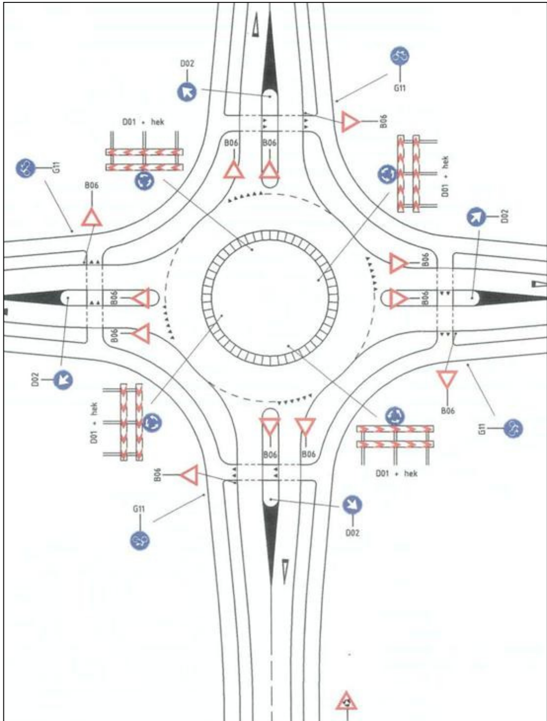
Figure 37: Signing for roundabouts in the Netherlands
