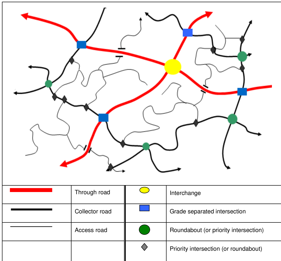
Figure 2: Categorization of a road network according to the sustainable safety concept
