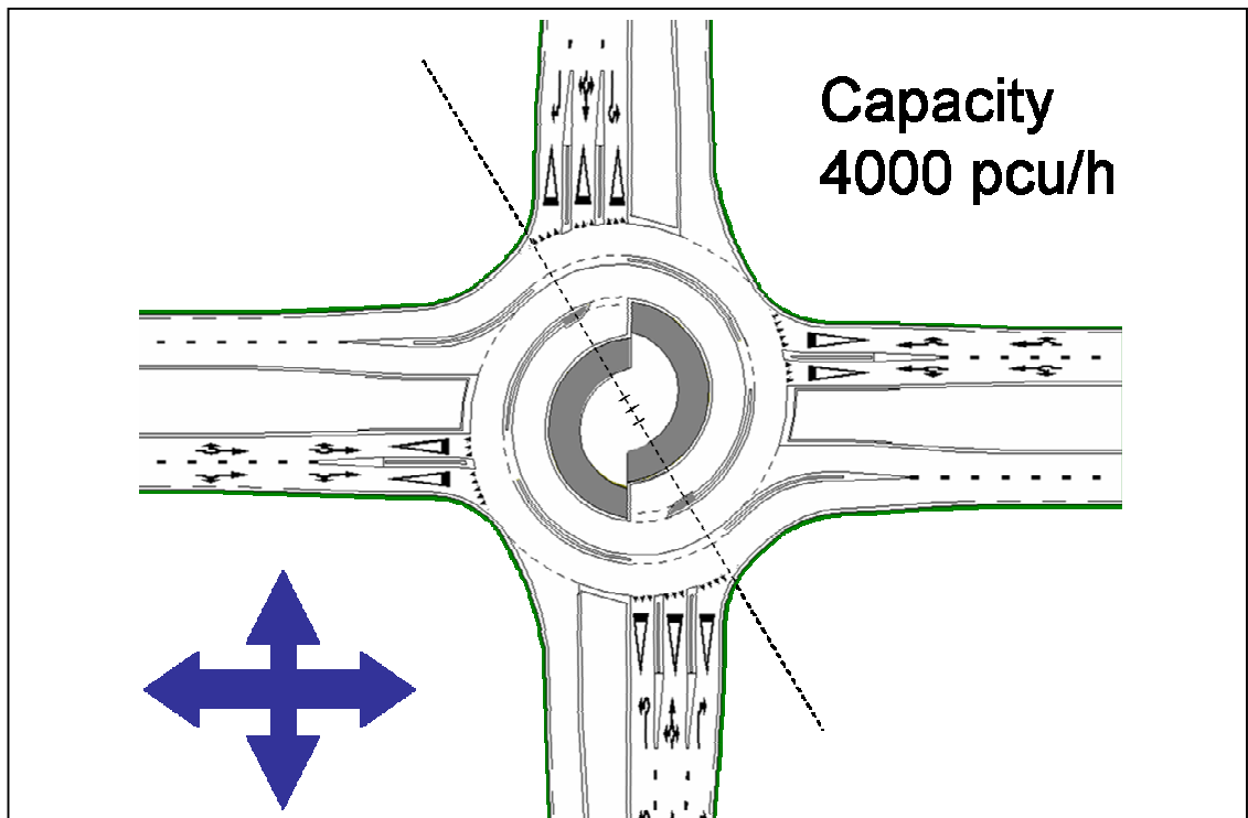
Figure 52: Spiral roundabout
