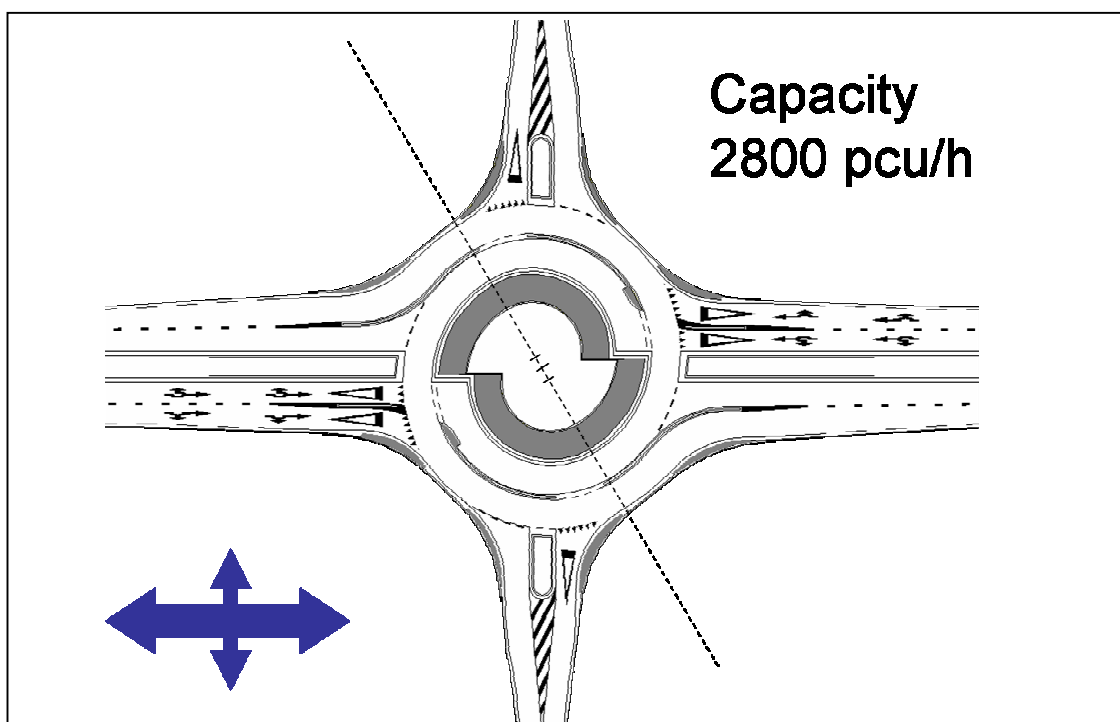
Figure 50: Egg roundabout
