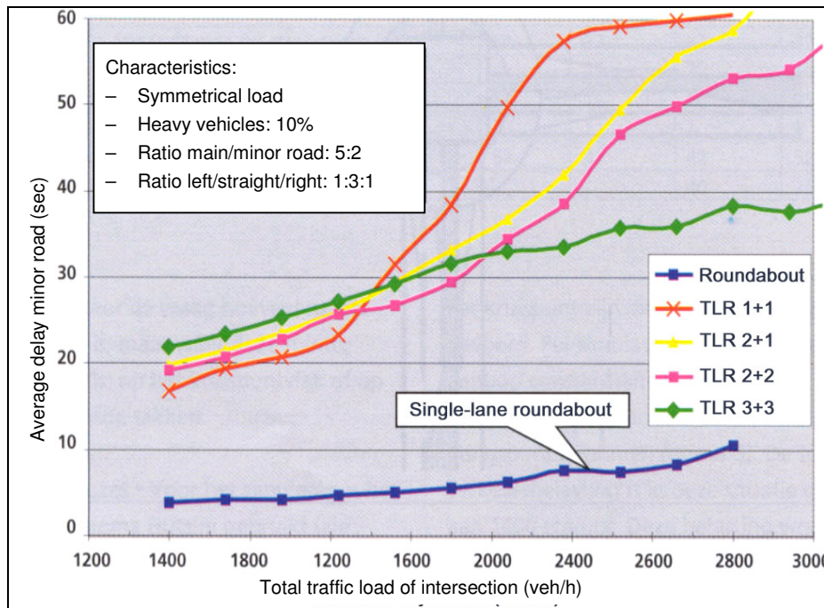
Figure 15: Average delay, minor road
