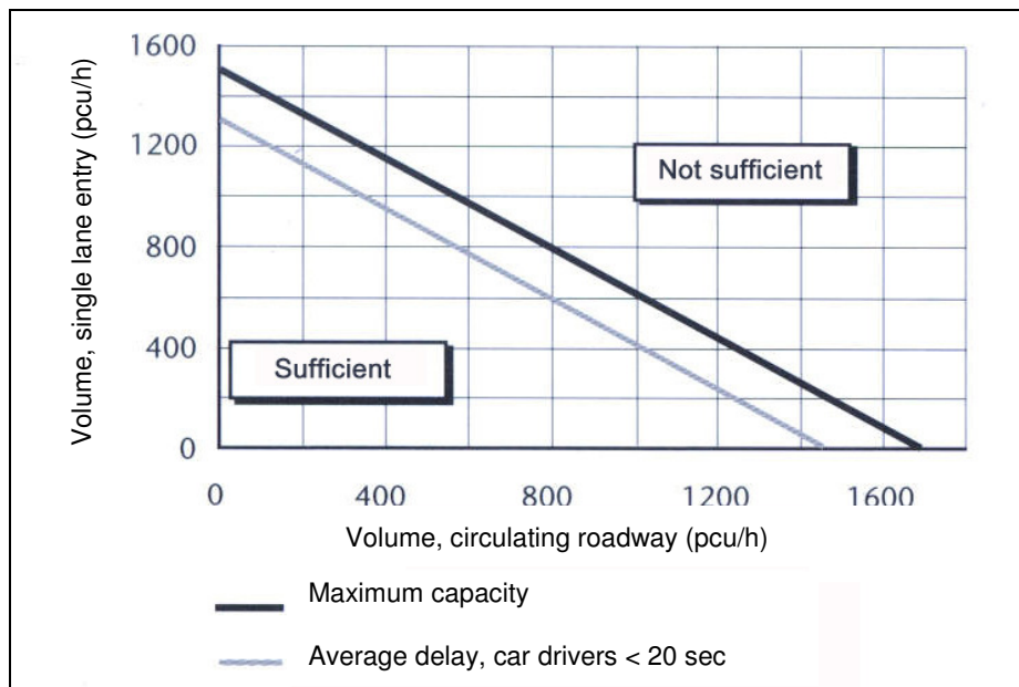
Figure 10: Nomogram capacity of a single lane roundabout with single lane entries (pedestrians and cyclists no priority), Bovy method
