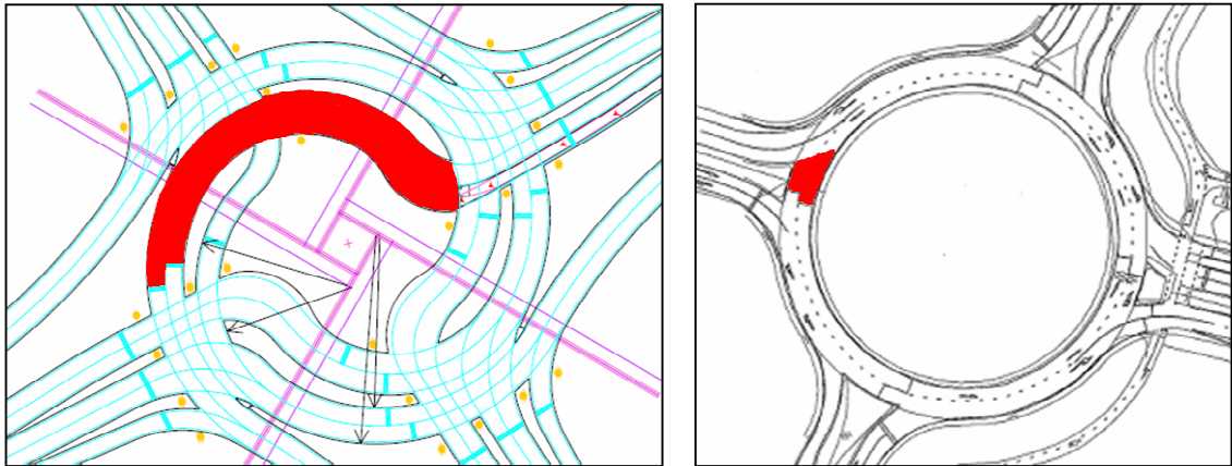
Figure 83: Buffer for left turning traffic: turbo roundabout versus multi lane roundabout
