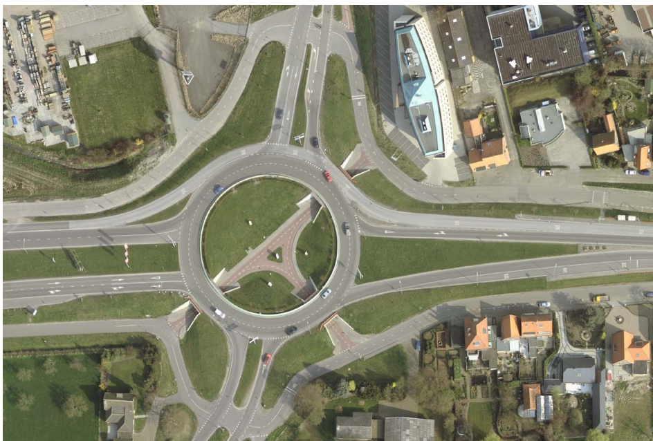
Figure 45: Example bicycle underpasses at a roundabout (the Netherlands)
