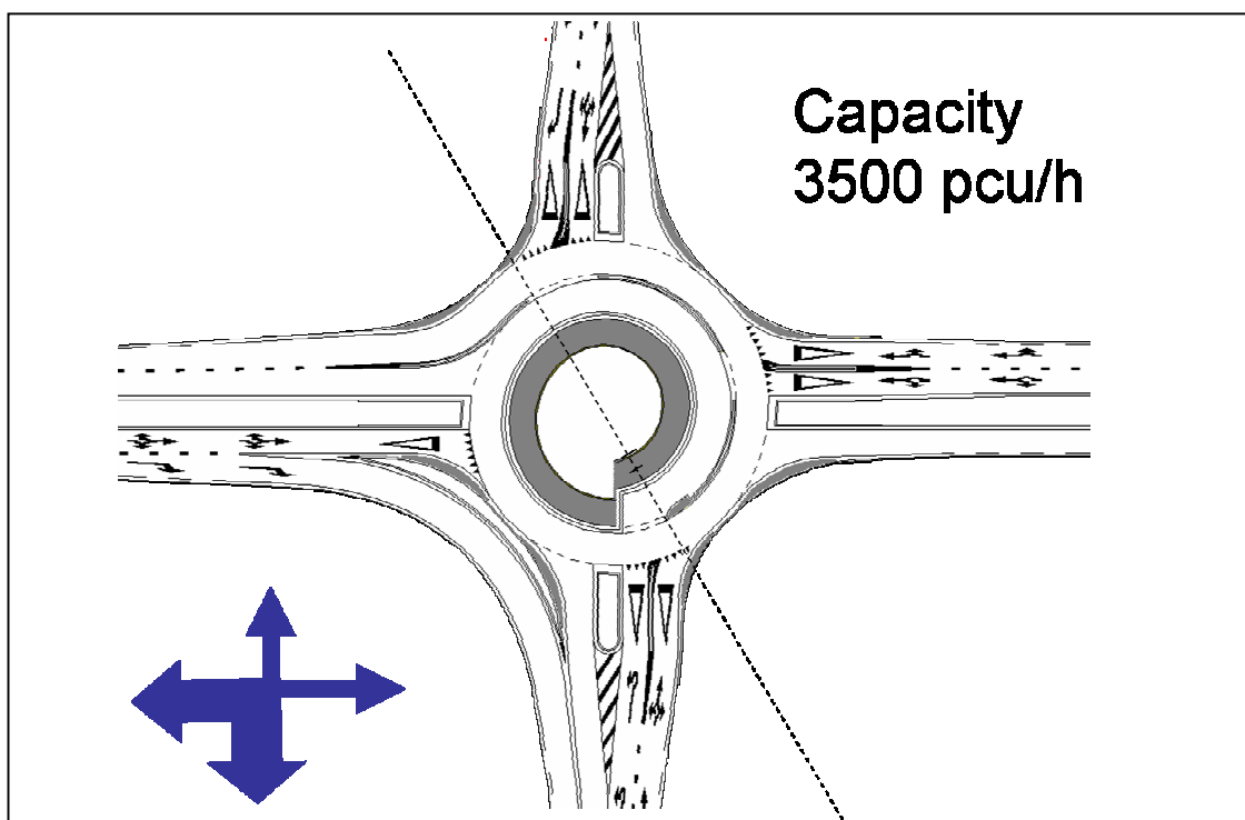
Figure 51: Knee roundabout
