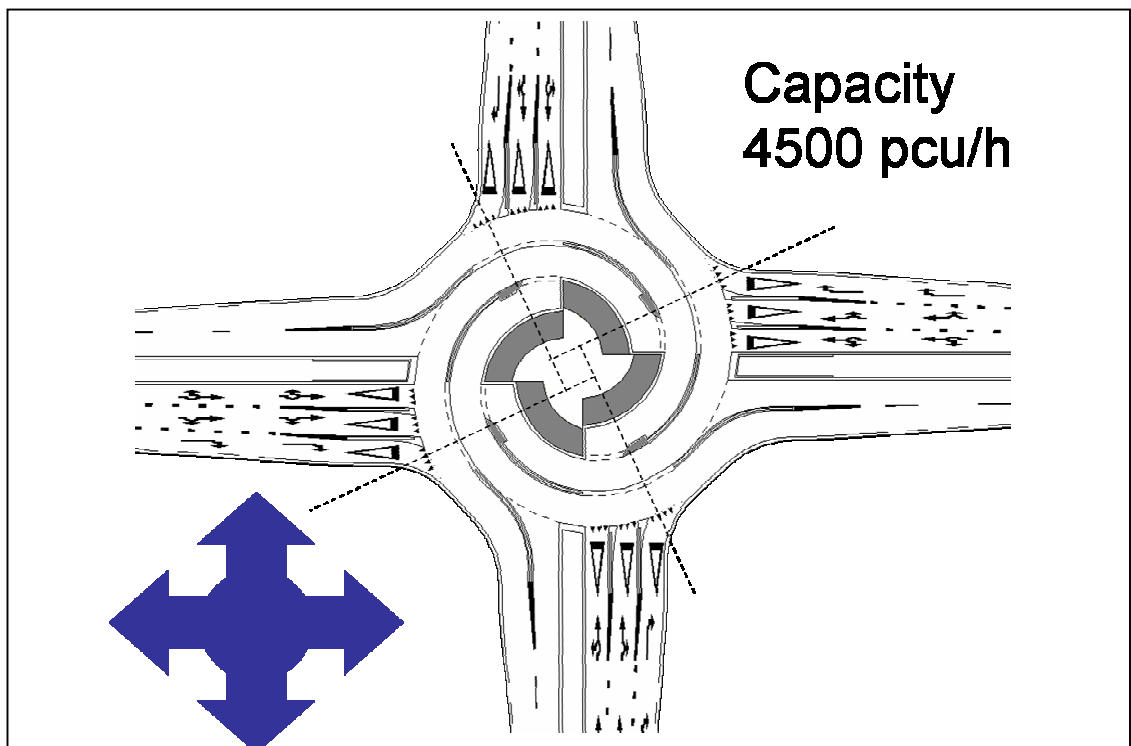
Figure 53: Rotor roundabout
