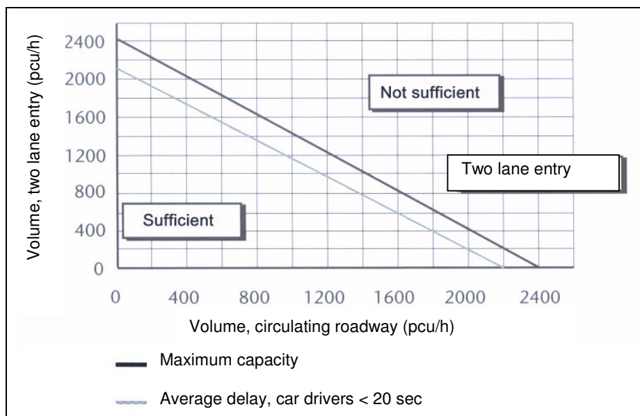
Figure 11: Nomogram capacity of a two lane roundabout with two lane entries (pedestrians and cyclists no priority), Bovy method
