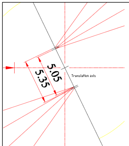
Figure 60: Detail showing centres for the arcs in a turbo roundabout
