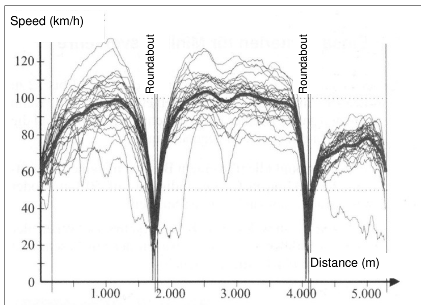
Figure 24: Speed characteristics on a road section with two roundabouts between two villages [13]
