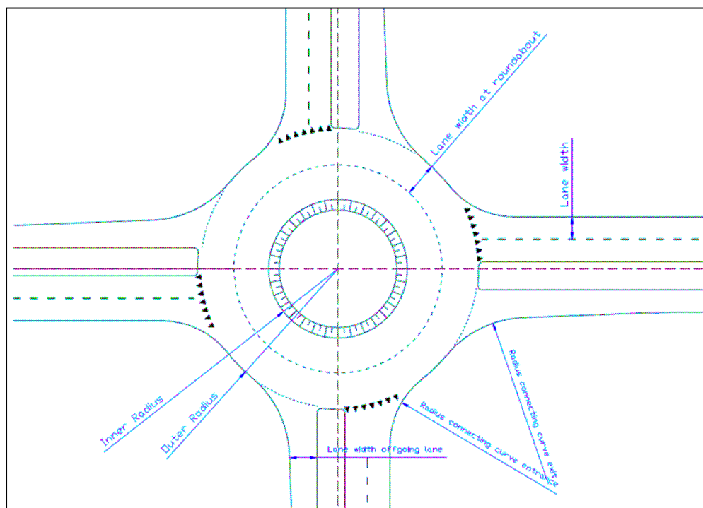
Figure 38: Former standard design multi lane roundabout in the Netherlands
