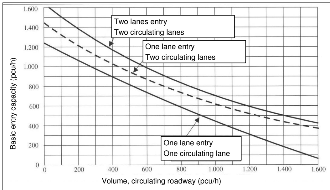
Figure 12: Basic capacity of entries (pedestrians and cyclists no priority), German method
