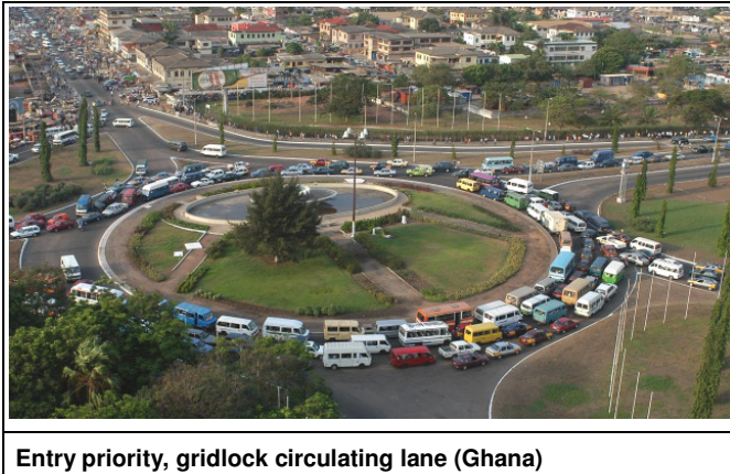
Figure 6: Consequences of priority rules on roundabouts
